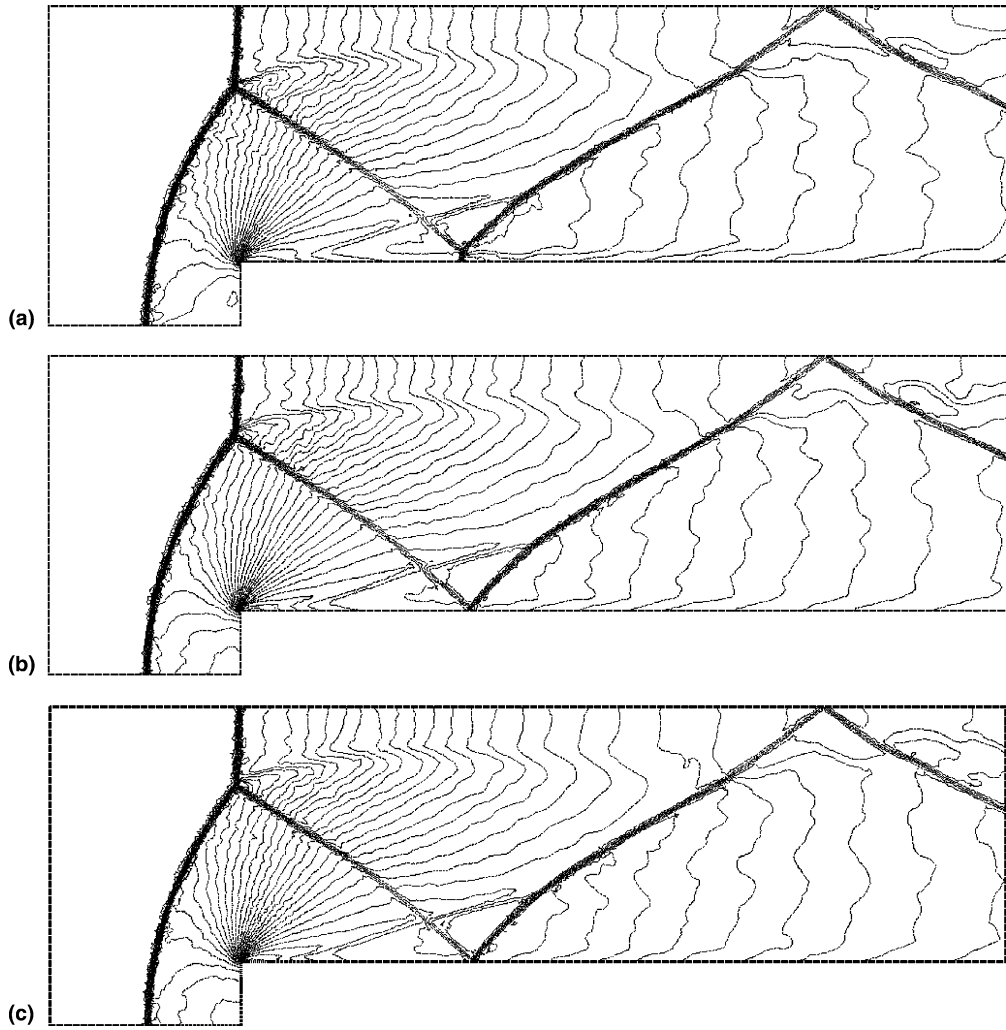
Fig. 15. Computed density contours with the third-order SV scheme using the Rusanov flux and TVD limiter.
